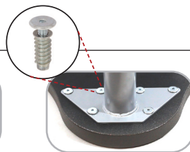
Legs positioned at widest point of table for stability and attached via threaded metal inserts and bolts
